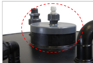
Hand hole with cable gland for level indicator
